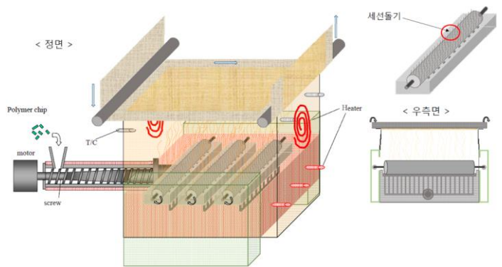
Melt-electro Spinning Apparatus for Mass Production of Nano-fiber(Drum Type)
